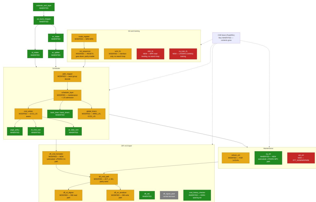
Figure 2.1: andesite DDR4/LPDDR4, inherited (green), modified (amber), new (red), dormant (grey)
