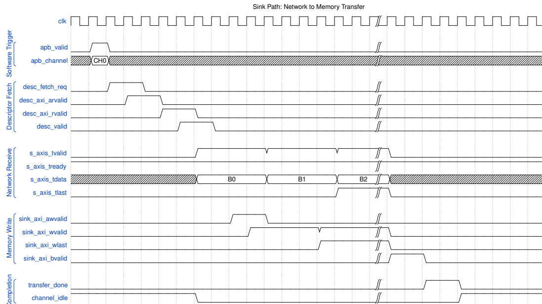
Timing Diagram
