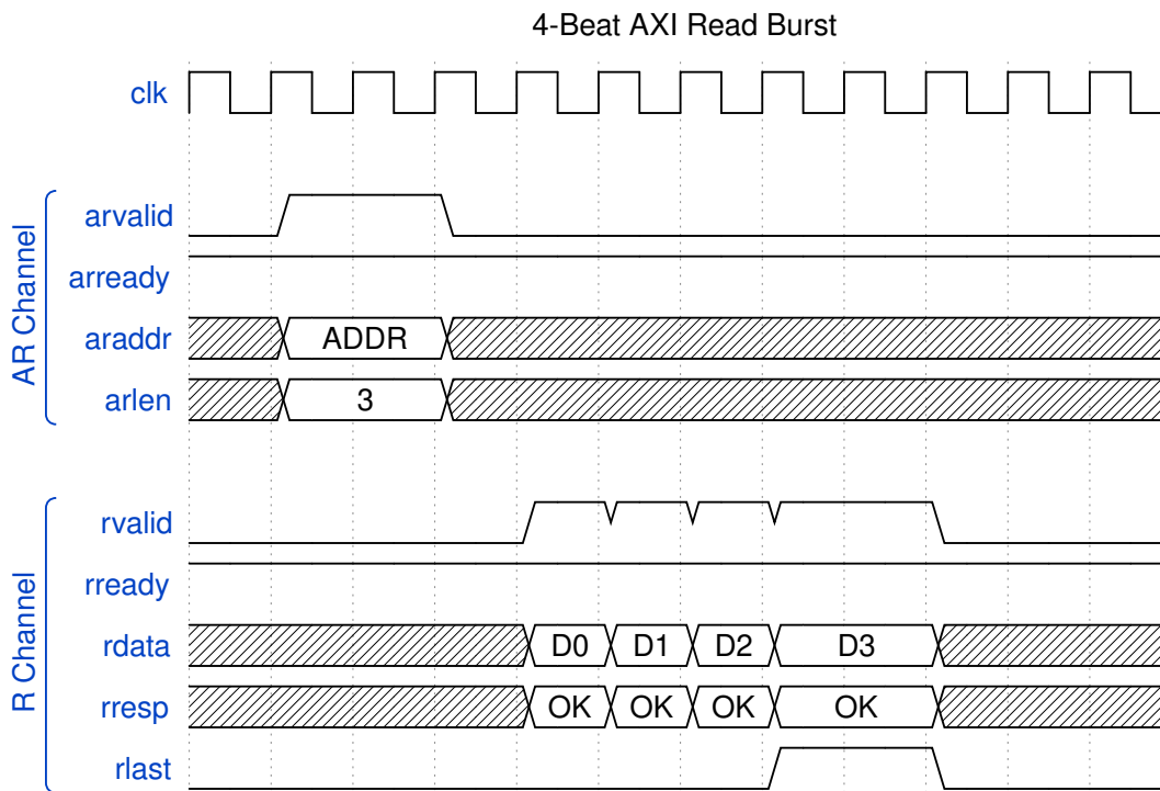
Timing Diagram
