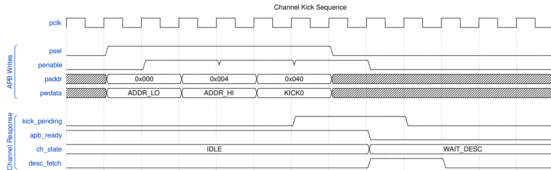
Waveform 33
