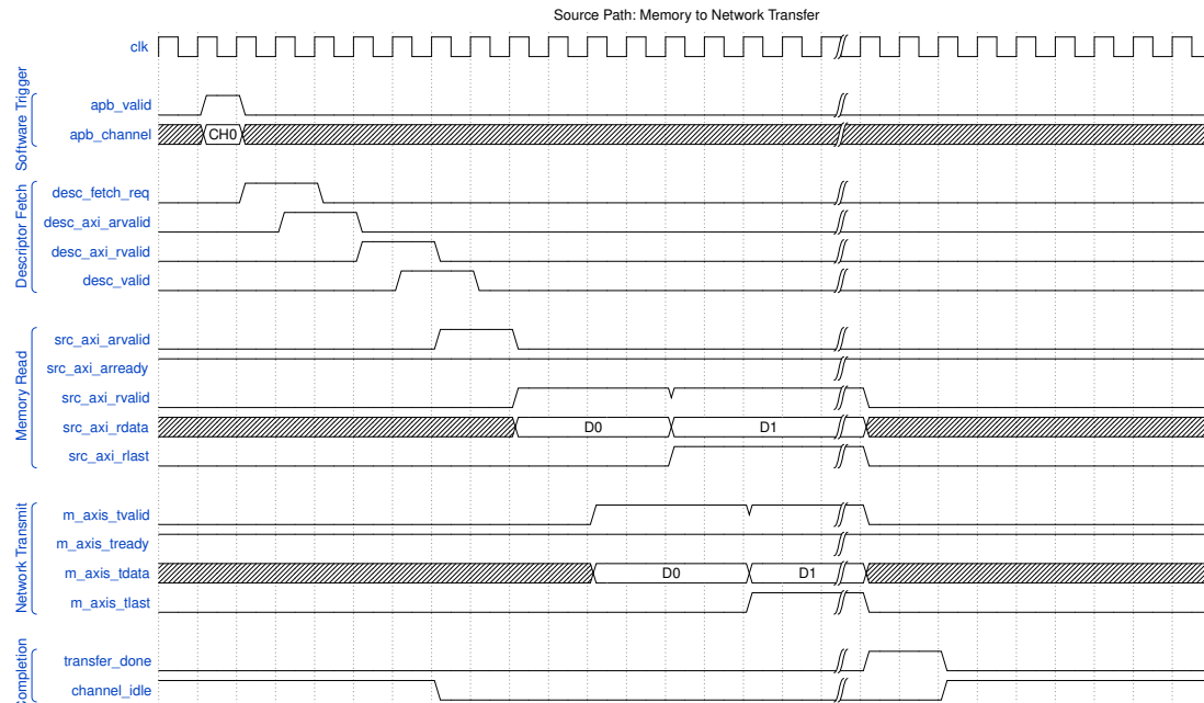
Timing Diagram
