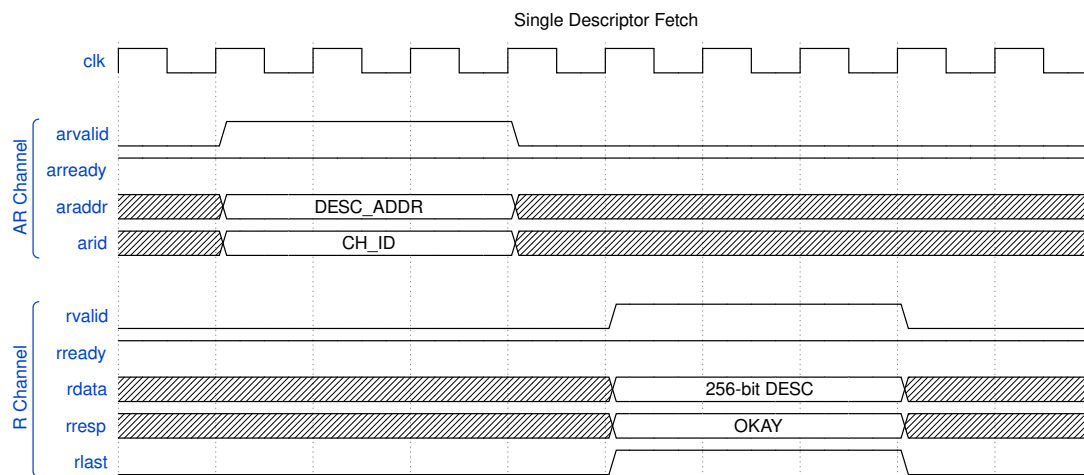
Timing Diagram
