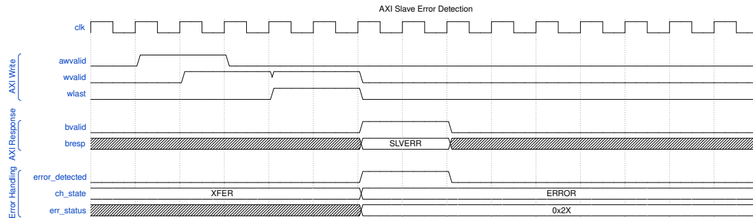
Waveform 36
