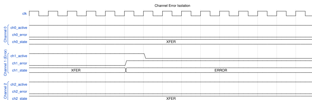
Waveform 27
