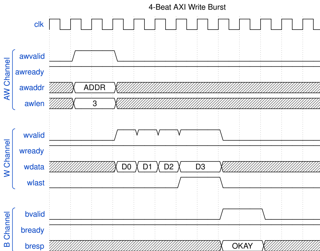
Timing Diagram
