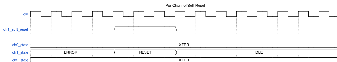
Waveform 28
