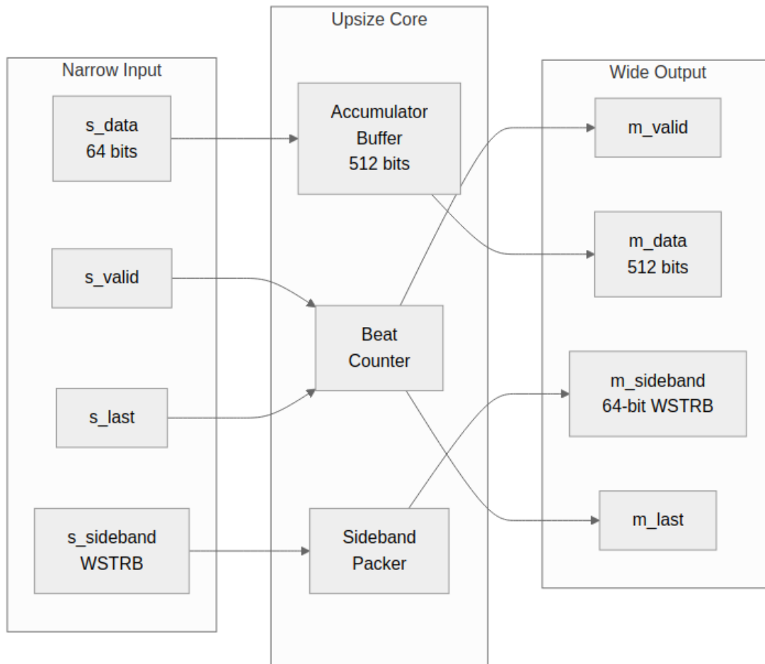
axi_data_upsize Architecture
