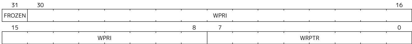
Figure 129. Supervisor Control Transfer Records Status Register Format
