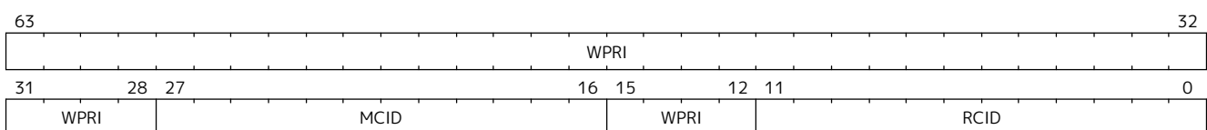
Figure 133. Supervisor Resource Management Configuration ( srmcfg ) register for SXLEN=64
