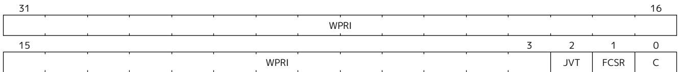
Figure 121. Supervisor State Enable 0 Register ( sstateen0 )
