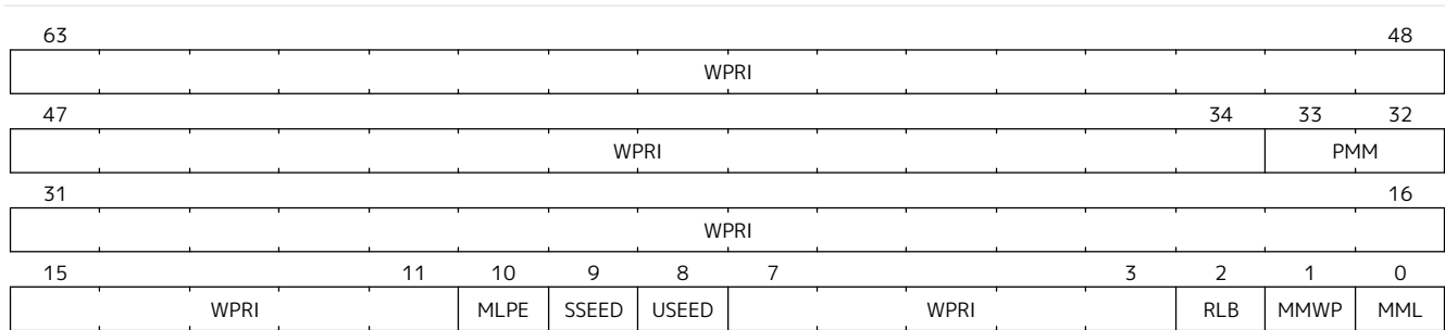
Figure 35. Machine security configuration ( mseccfg ) register.
