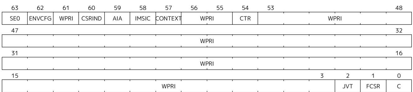
Figure 120. Hypervisor State Enable 0 Register ( hstateen0 )
