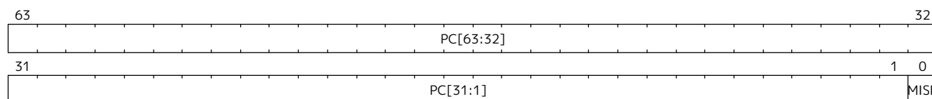
Figure 131. Control Transfer Record Target Register Format for MXLEN=64
