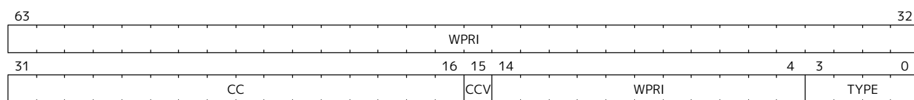
Figure 132. Control Transfer Record Metadata Register Format
