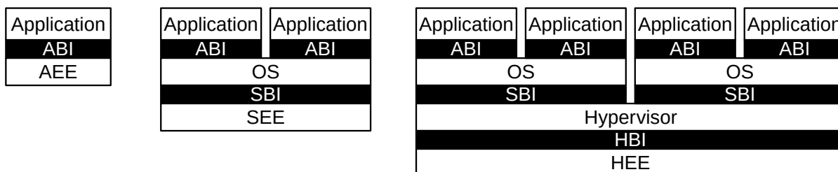
Figure 10. Different implementation stacks supporting various forms of privileged execution.
