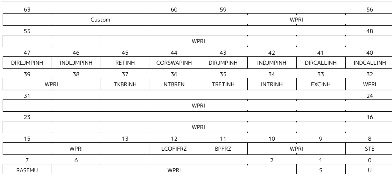
Figure 127. Virtual Supervisor Control Transfer Records Control Register Format
