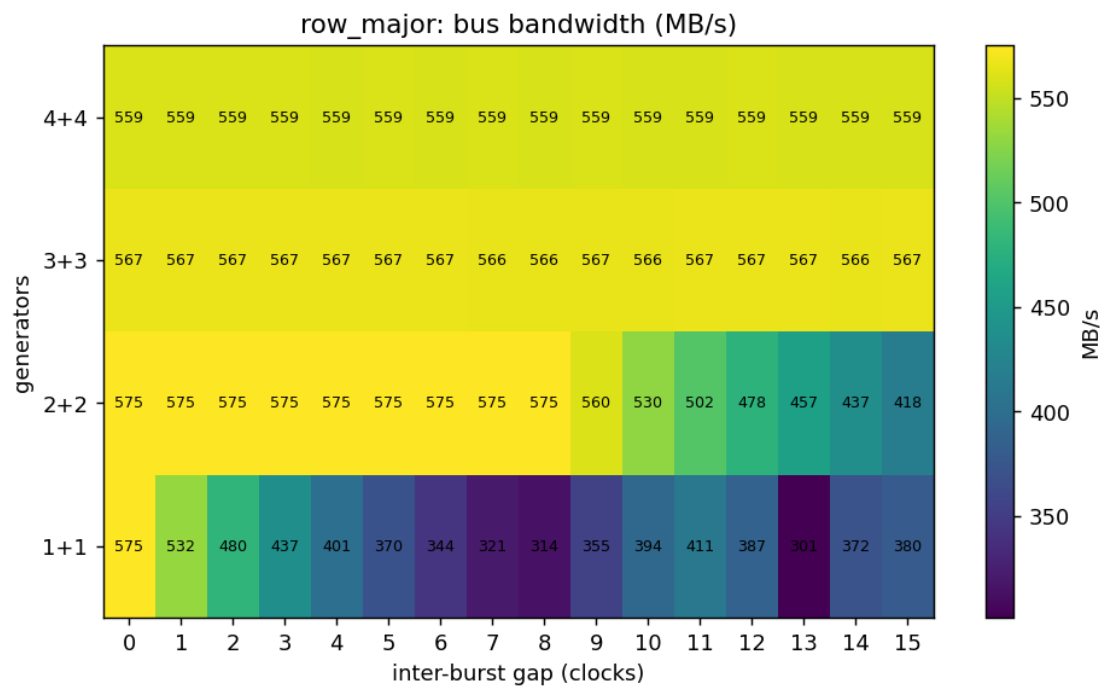
Heatmap of total bus bandwidth against gap and generator count, row-major
