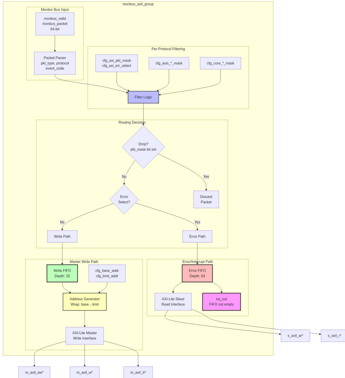
MonBus AXI-Lite Group Block Diagram
