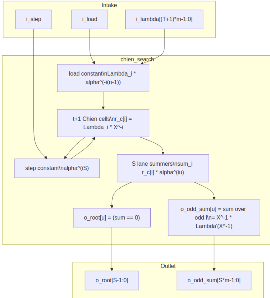
Chien search block diagram
