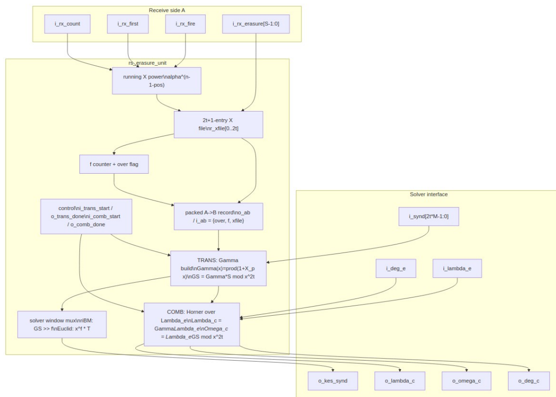
11.1.1 Figure 2.7: Erasure unit block diagram
