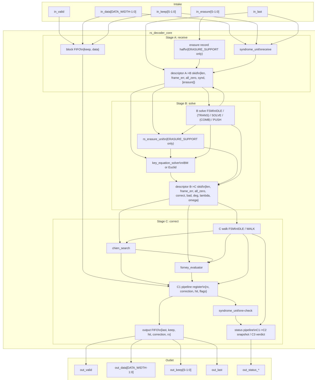
Decoder core block diagram
