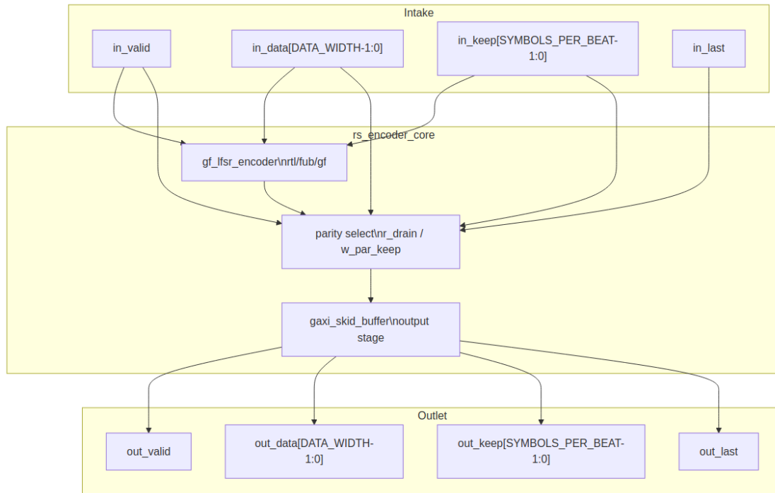
Encoder core block diagram
