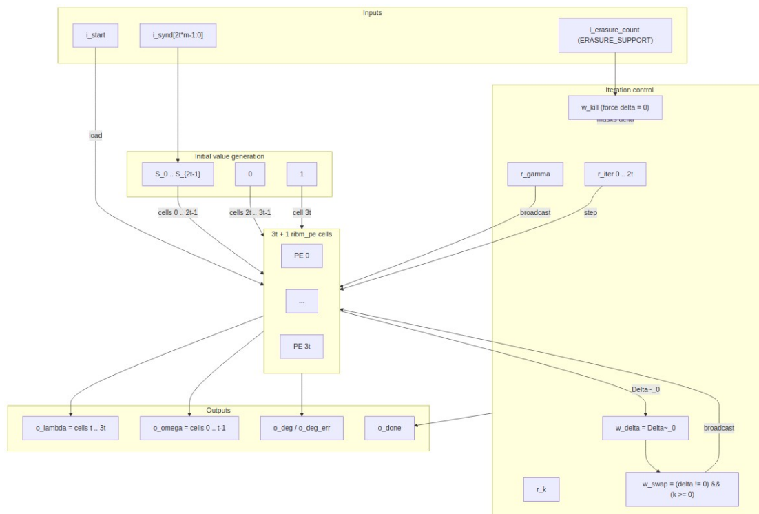
7.1.1 Figure 2.3: riBM solver block diagram
