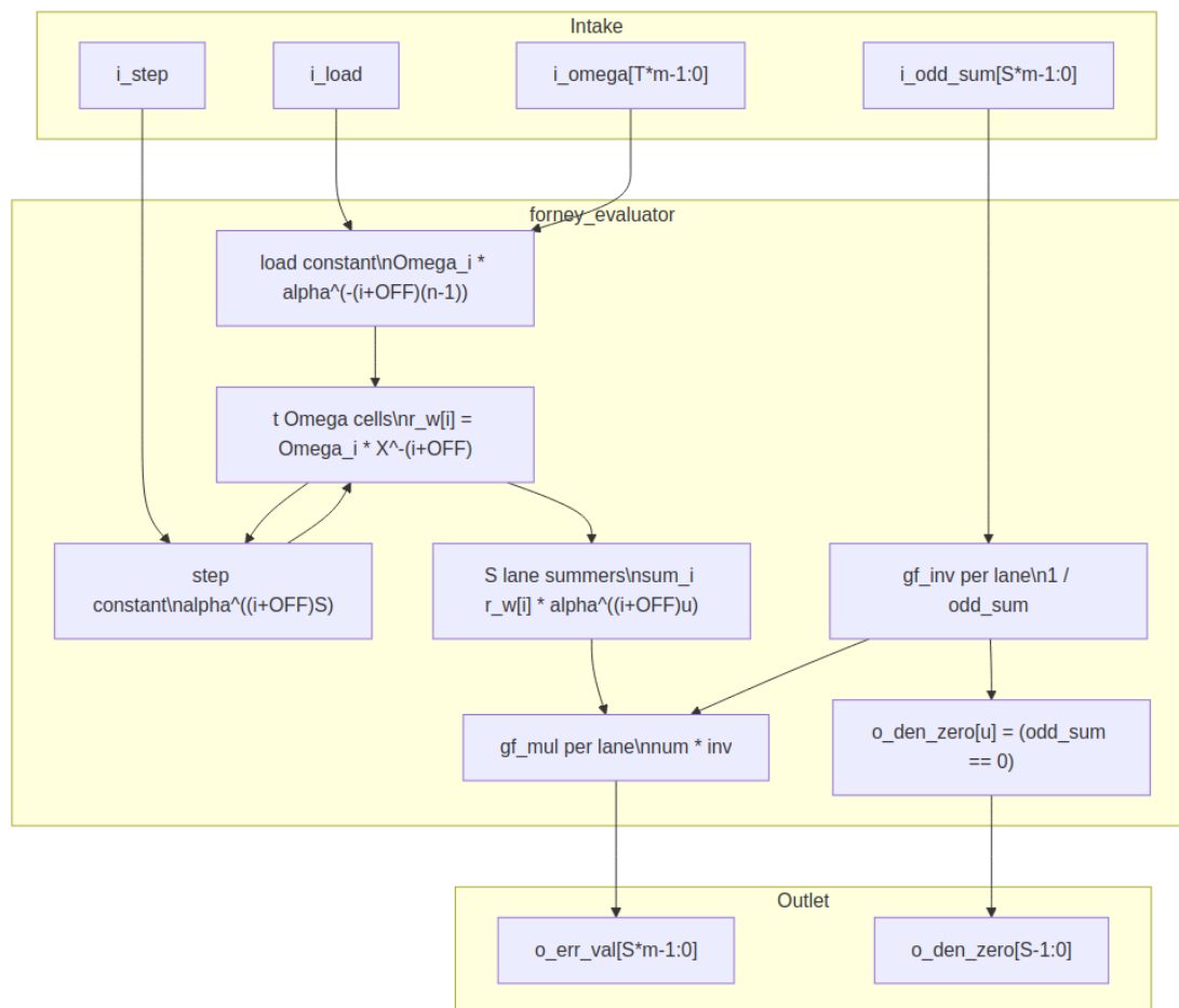
Forney evaluator block diagram
