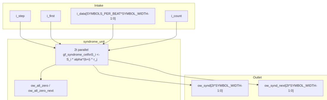
Syndrome unit block diagram
