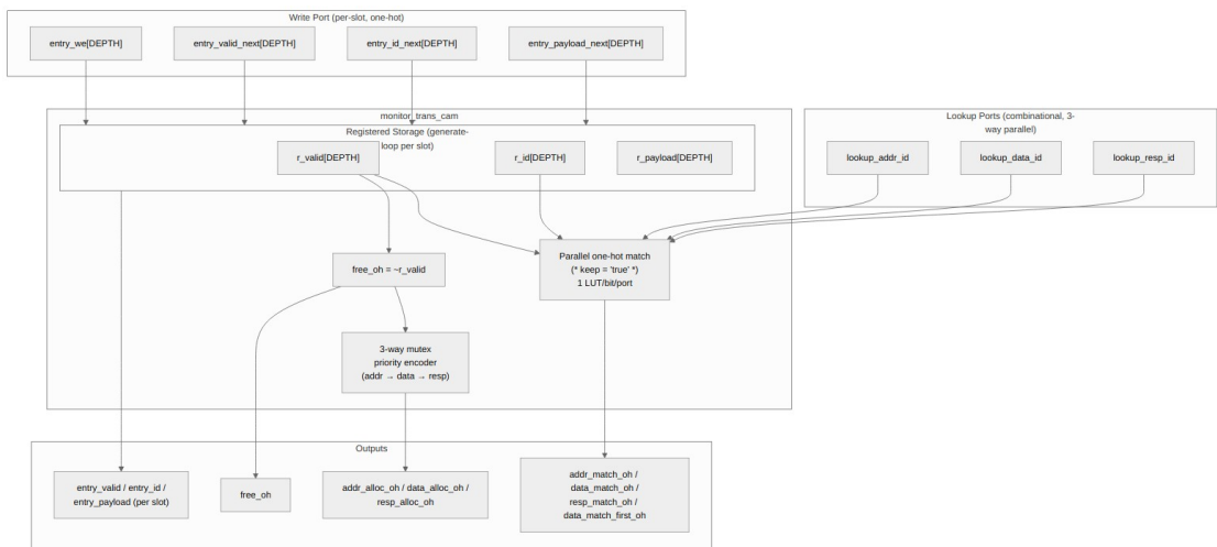
monitor_trans_cam block diagram
