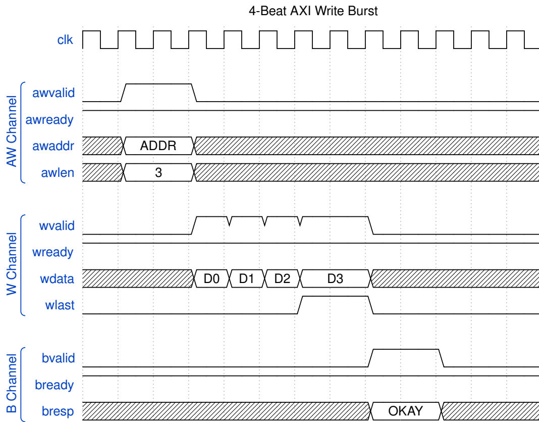
Timing Diagram
