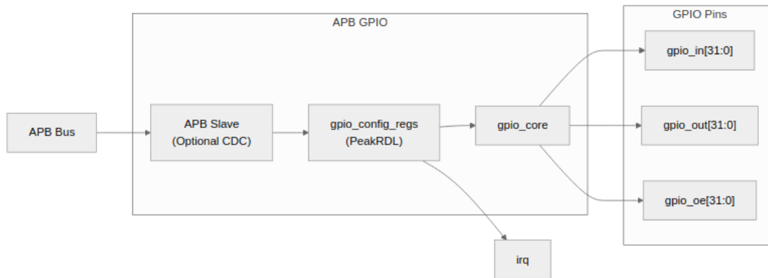
APB GPIO Block Diagram
