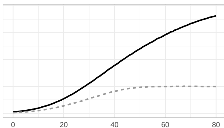
F 6 Cauchy
