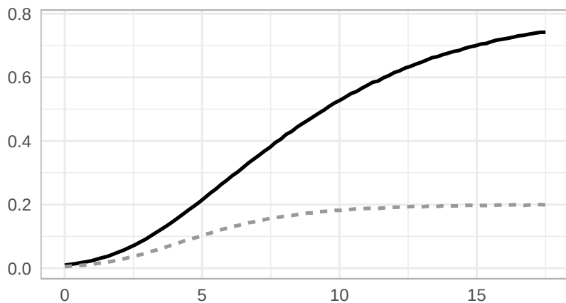
F 5 Logistic
