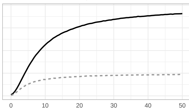
F 8 Exponential
