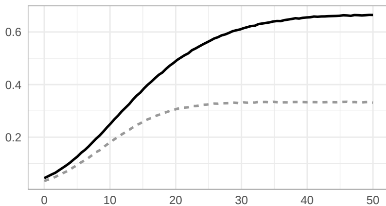
F 3 Normal with outliers
