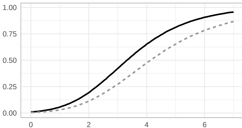
F 5 Logistic
