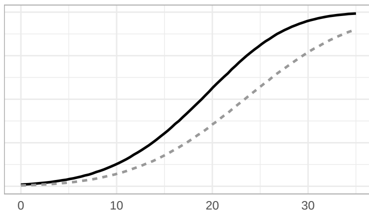
F 6 Cauchy
