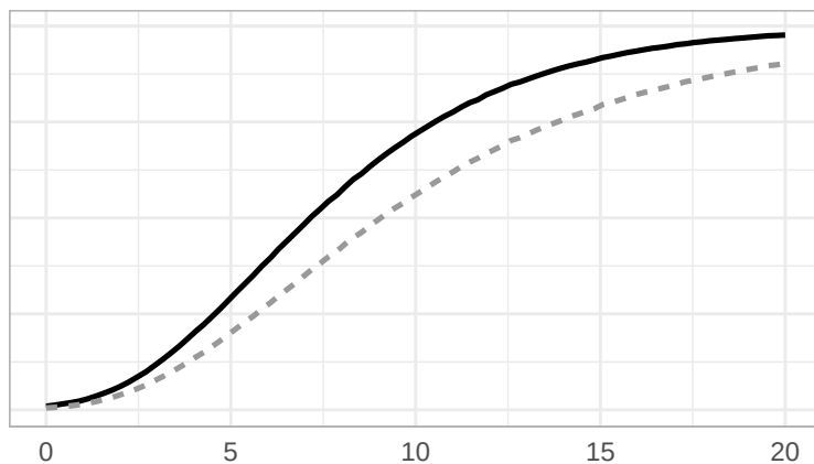
F 8 Exponential
