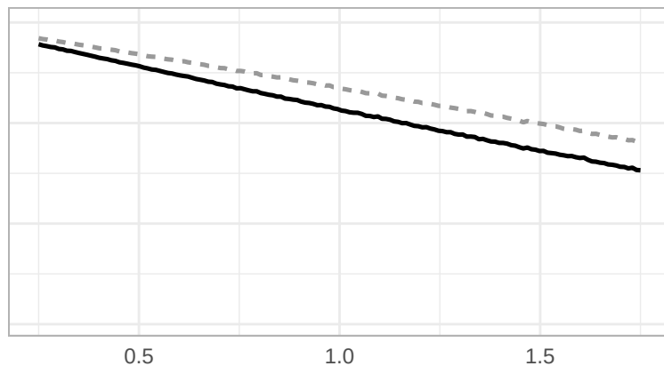
F_8(\sigma^2) Exponential family (with shift d=7.5 )
