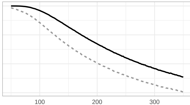
F_4(\sigma^2) Normal plus uniform family (with shift d=15 )
