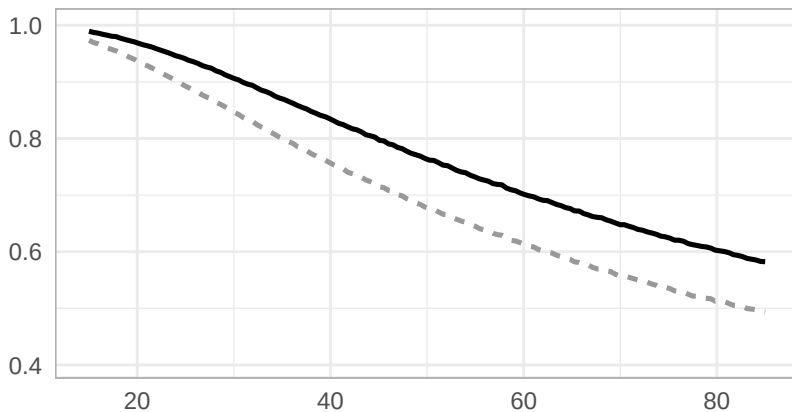
F_7(\sigma^2) Gumbel family (with shift d=7.5 )
