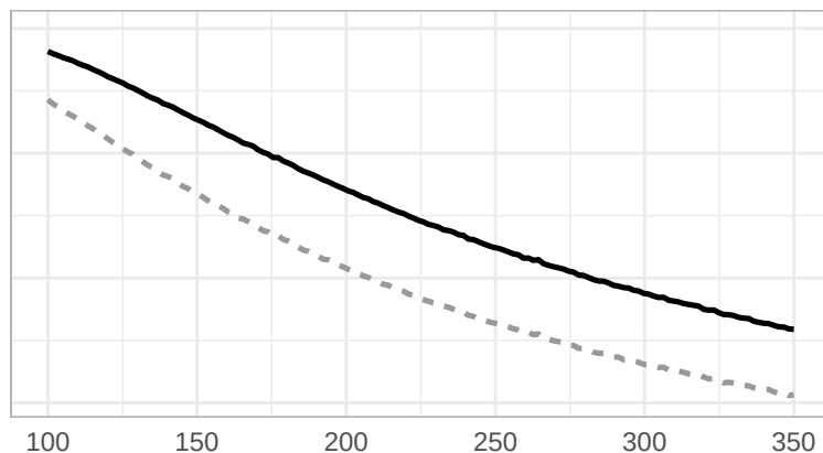
F_6(\sigma^2) Cauchy family (with shift d=7.5 )
