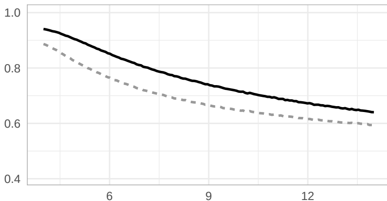
F_5(\sigma^2) Logistic family (with shift d=7.5 )
