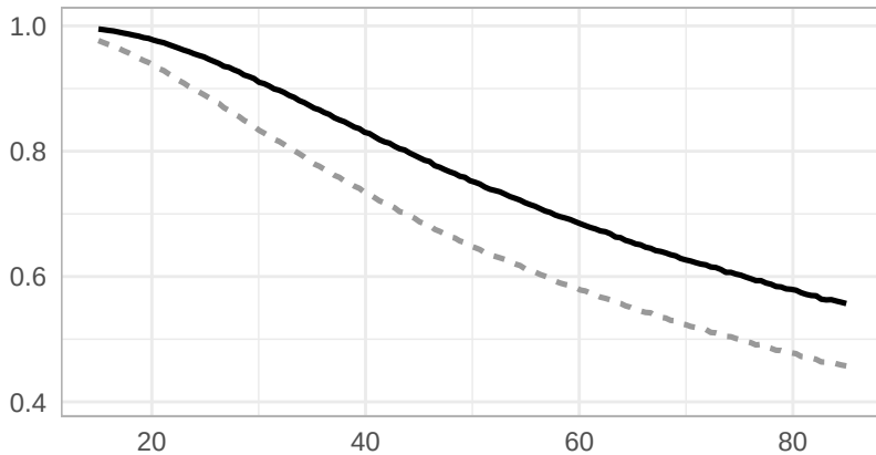
F_3(\sigma^2) Normal with outliers family (with shift d=3 )
