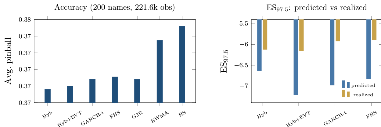
Figure OA.4: The FRTB battery. Left: average pinball loss by model (axis truncated to resolve the ordering; differences carry DM 5.6–9.7 vs the hybrid, all p \approx 0 ); CAViaR, not shown, statistically ties the hybrid. Right: ES_{97.5} predicted (exact tail integral) vs realized below each model’s own VaR, a model-dependent diagnostic, not a ranking (every fat-tailed entrant’s integral exceeds its own-tail mean); the joint FZ0 score of the paper is the ranking criterion.
