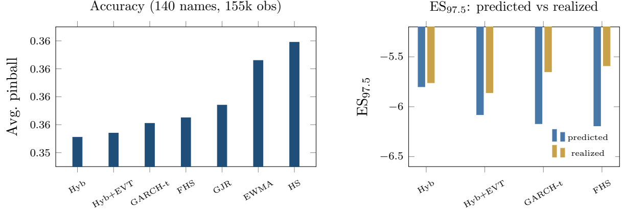
Figure 4: The FRTB battery. Left: average pinball loss by model (axis truncated to resolve the ordering; differences carry DM 4.4–8.3 vs the hybrid, all p \approx 0 ); CAViaR, not shown, statistically ties the hybrid. Right: ES_{97.5} predicted vs realized — FHS and GARCH- t over-state ES by 8–11% (over-charging capital) while the hybrid is nearly exact.
