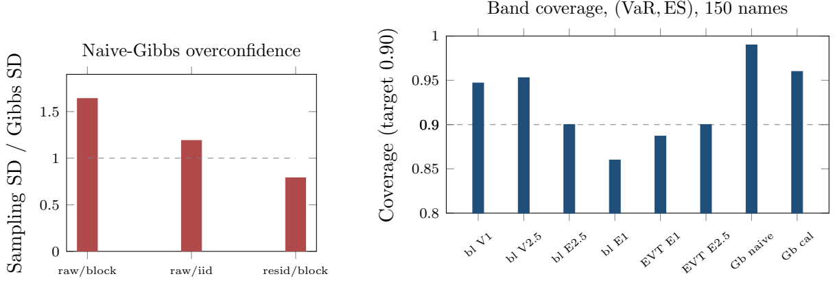
Figure 6: Honest uncertainty, assembled. Left: the naive Gibbs posterior SD understates the block-bootstrap sampling SD 1.64\times on raw returns (i.i.d. bootstrap 1.19 — the gap is the dependence contribution); the ratio falls to 0.79 on GARCH residuals. Right: coverage of nominal-90% bands (bl = block bootstrap; V = VaR, E = ES at the stated level; Gb = Gibbs, naive \omega vs \omega -calibrated). Block bootstrap and the EVT interval sit at or near target; the naive Gibbs over-covers.
