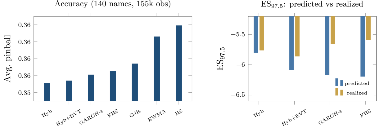
Figure 6: The FRTB battery. Left: average pinball loss by model (axis truncated to resolve the ordering; differences carry DM 4.4–8.3 vs the hybrid, all p \approx 0 ); CAViaR, not shown, statistically ties the hybrid. Right: ES_{97.5} predicted vs realized — FHS and GARCH- t over-state ES by 8–11% (over-charging capital) while the hybrid is nearly exact.
