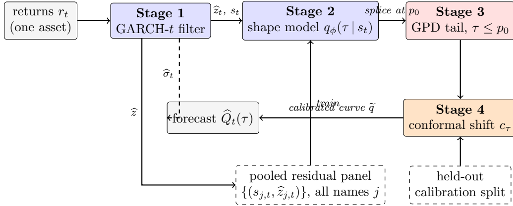
Figure OA.7: The residual-hybrid estimator as a pipeline (Section 3 of the paper). Solid arrows carry data; the dashed top arrow carries the conditional scale \hat{\sigma}_t that rescales the finished residual quantile curve. Dashed boxes are inputs shared across assets (the pooled panel that trains the amortized shape model) or held out from training (the calibration split behind the conformal overlay).
