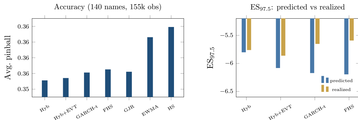
Figure OA.4: The FRTB battery. Left: average pinball loss by model (axis truncated to resolve the ordering; differences carry DM 4.4–8.3 vs the hybrid, all p \approx 0 ); CAViaR, not shown, statistically ties the hybrid. Right: ES 97.5 predicted vs realized — FHS and GARCH- t over-state ES by 8–11% (over-charging capital) while the hybrid is nearly exact.
