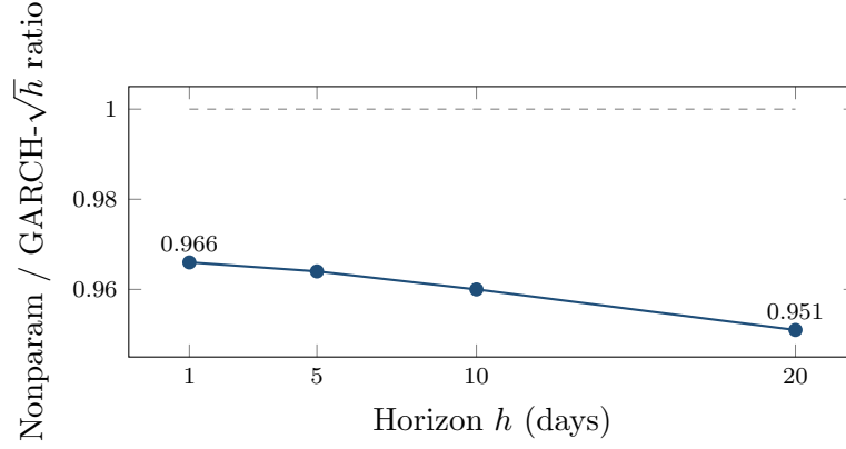
Figure OA.3: The edge grows with horizon. Nonparametric/GARCH pinball ratio at h = 1, 5, 10, 20 days (amortized panel): fat tails compound while \sqrt{h} scaling compounds the shape error — \sim 5\% at h = 20 . Direct-learning design: a fresh quantile model per horizon against \sqrt{h} -scaled GARCH- t ; the deployed engine’s own ten-day numbers in the main text ( 0.4\% \rightarrow 1.4\% ) come from the stress battery and are smaller — the designs differ and are labeled where quoted.
