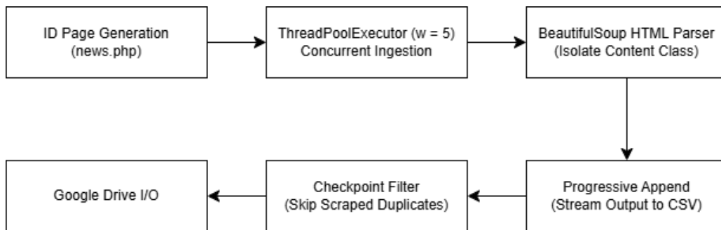
Figure X: Web Crawler Methodology
