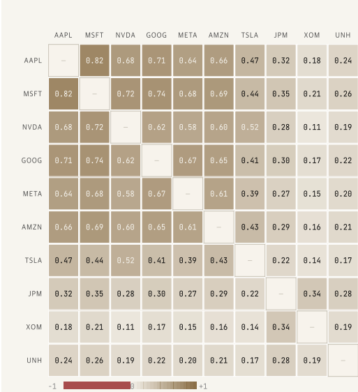
Fig. 1. Ninety-day rolling Pearson correlation on log returns. Bronze · positive co-movement. Faint red · negative. The diagonal is omitted so the eye reads pairs, not self-references.
