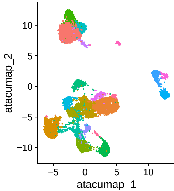
ATAC only
