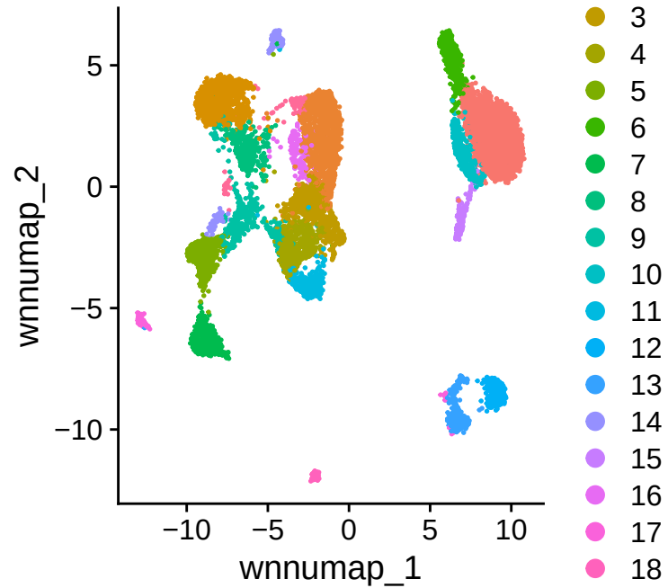
WNN (joint)
