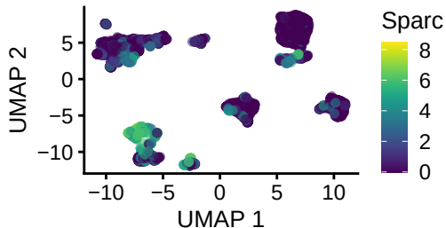
cluster 12 – Sparc
