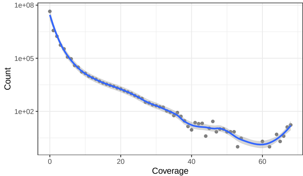
Chromosome chr22
