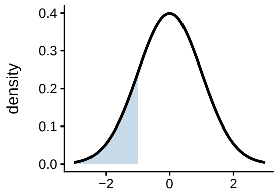
\text{pnorm}(-1) = 0.16
