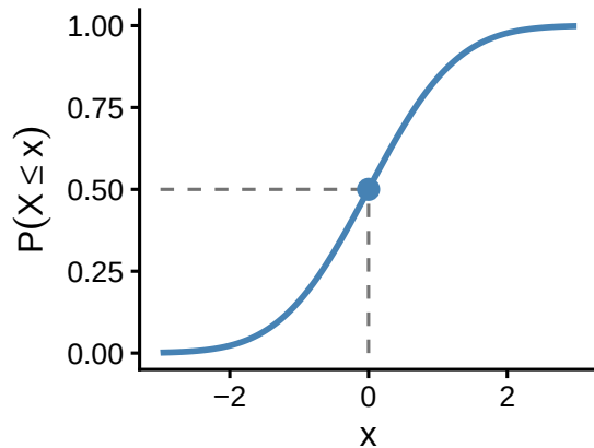
\text{pnorm}(0) = 0.50
