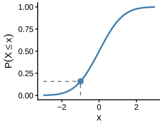
\text{pnorm}(-1) = 0.16
