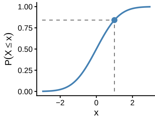
\text{pnorm}(1) = 0.84
