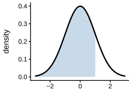
\text{pnorm}(1) = 0.84
