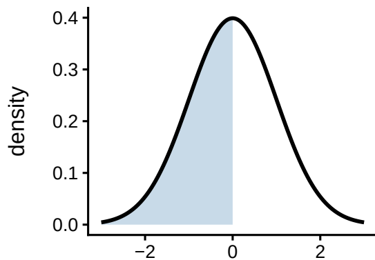
\text{pnorm}(0) = 0.50
