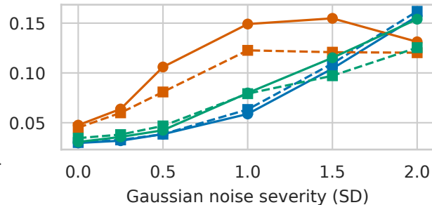
Breast Cancer
