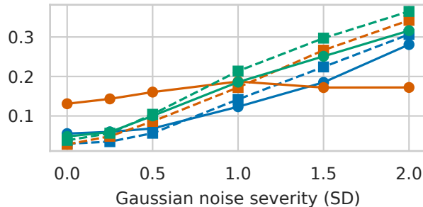
Wine
