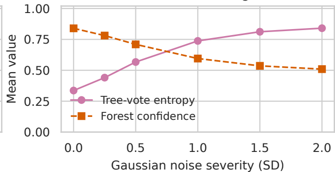
(c) Random-forest disagreement
