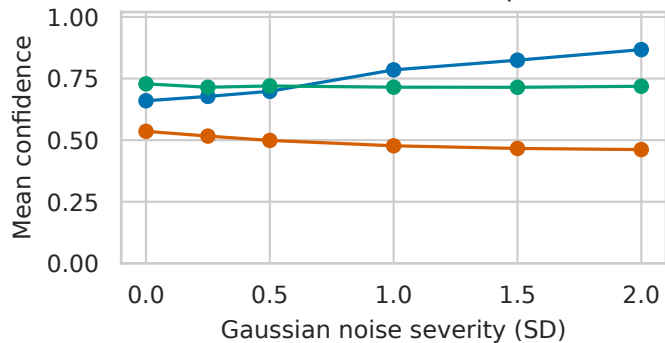
(a) Confidence on incorrect predictions
