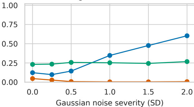
(b) High-confidence errors
