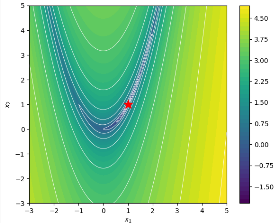
Rosenbrock (curved valley, non-convex) ( d = 2 )
