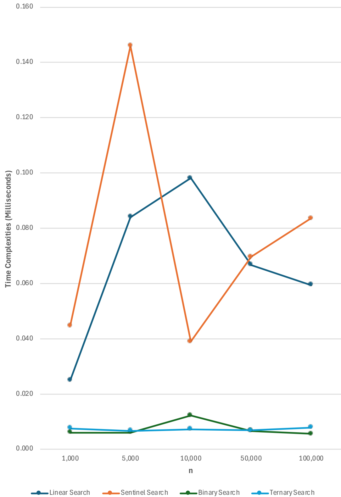
Search Algorithms Efficiency Comparison
