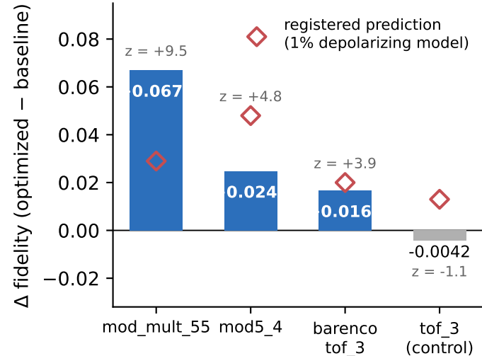
(a) one interleaved job per pair, 8192 shots
