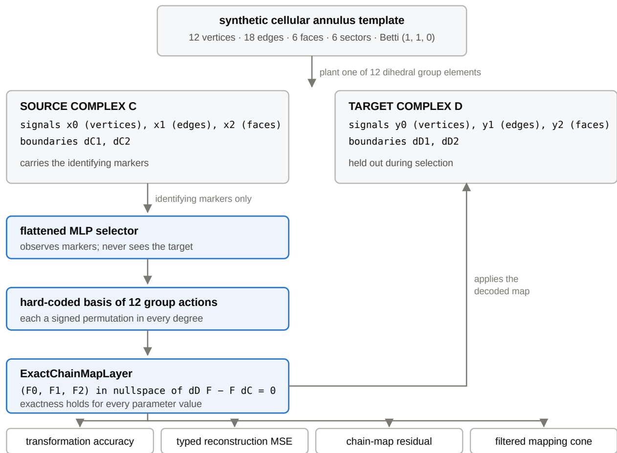
Figure 1. Architecture and data flow. A group element is planted in the annulus template. The selector observes only the identifying markers and never sees the target complex. It chooses one member of a fixed twelve-element basis, and the resulting typed map is scored four ways. The chain-map constraint is structural — it holds for every parameter value — so the residual is a numerical check, not a learned objective.
