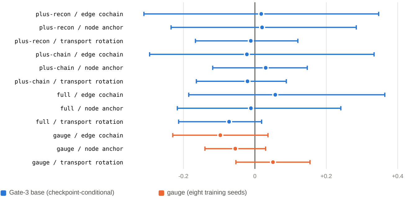
Figure 4. Every corruption contrast interval contains zero. Candidate minus baseline on the adjusted partial-Spearman endpoint. The nine Gate-3 base contrasts use a paired complete-block bootstrap and are conditional on a fixed checkpoint pair; the three gauge contrasts use a Student-t interval with df = 7 across eight training seeds. No multiplicity adjustment is applied. Generated from results/gate3/paired_comparison_final.json and results/summaries/gauge-corruption-campaign.json .
