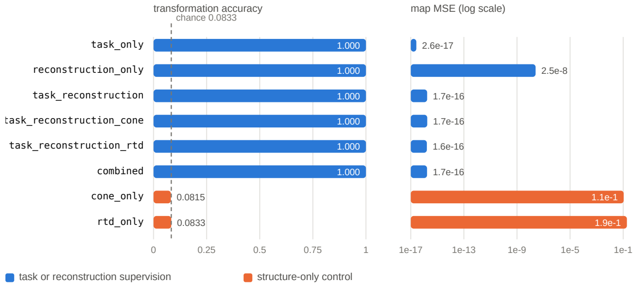
Figure 2. Exact recovery by training objective. Mean over five seeds; every declared ablation is shown, grouped as supervised objectives then identifiability controls. Left: transformation accuracy against the 0.0833 chance baseline. Right: map mean-squared error on a log scale. Any objective carrying task or reconstruction supervision saturates; the two structure-only controls sit at chance with map errors fifteen orders of magnitude larger. Generated from results/summaries/identifiable-campaign-summary.json .
