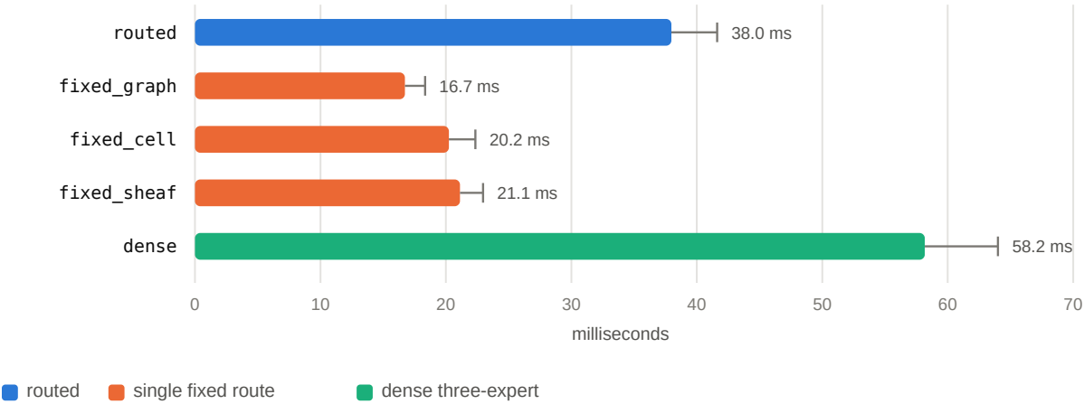
Figure 3. Trained routing inference latency on GB10. Median over 100 timed iterations, averaged across five seeds; whiskers mark mean p95. Batch 64, bfloat16. Routed inference is faster than dense evaluation and slower than any single fixed route. All paths were timed in the plotted order inside one process, so residual thermal or allocator drift is confounded with path order. Generated from results/summaries/compute-campaign.json .
