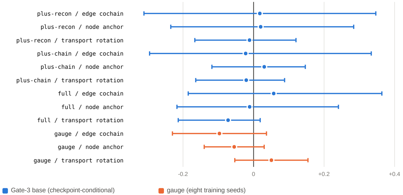
Figure 6. Every corruption contrast interval contains zero. Nine Gate-3 base contrasts use a paired complete-block bootstrap conditional on a fixed checkpoint pair; three gauge contrasts use a Student-t interval with df = 7 across eight training seeds. No multiplicity adjustment. Generated from results/gate3/paired_comparison_final.json and results/summaries/gauge-corruption-campaign.json .
