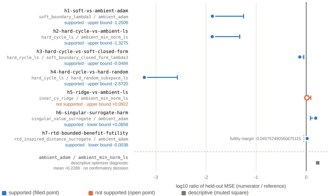
Figure 3. The seven-claim family of the sealed untouched-seed replication. Point: mean paired \log_{10} (held-out MSE, numerator arm / reference arm) over 33 eligible generator seeds; whisker: the governing one-sided Bonferroni bound in the claim's direction (familywise \alpha = 0.05/7 , critical value 2.5912722991315227). H5 (ridge) is not supported. The dashed marker on H7 is the prespecified futility margin \log_{10}(0.90) ; H7 is a bounded-benefit/futility statement only and cannot establish equality or the absence of every benefit. The muted square below the divider is the descriptive optimizer diagnostic (ambient Adam / ambient minimum-norm LS), which carries no support decision. Same-generator-family replication on synthetic seeds, not real-data validation. Generated from results/campaigns/lifting-replication-v2.json .
