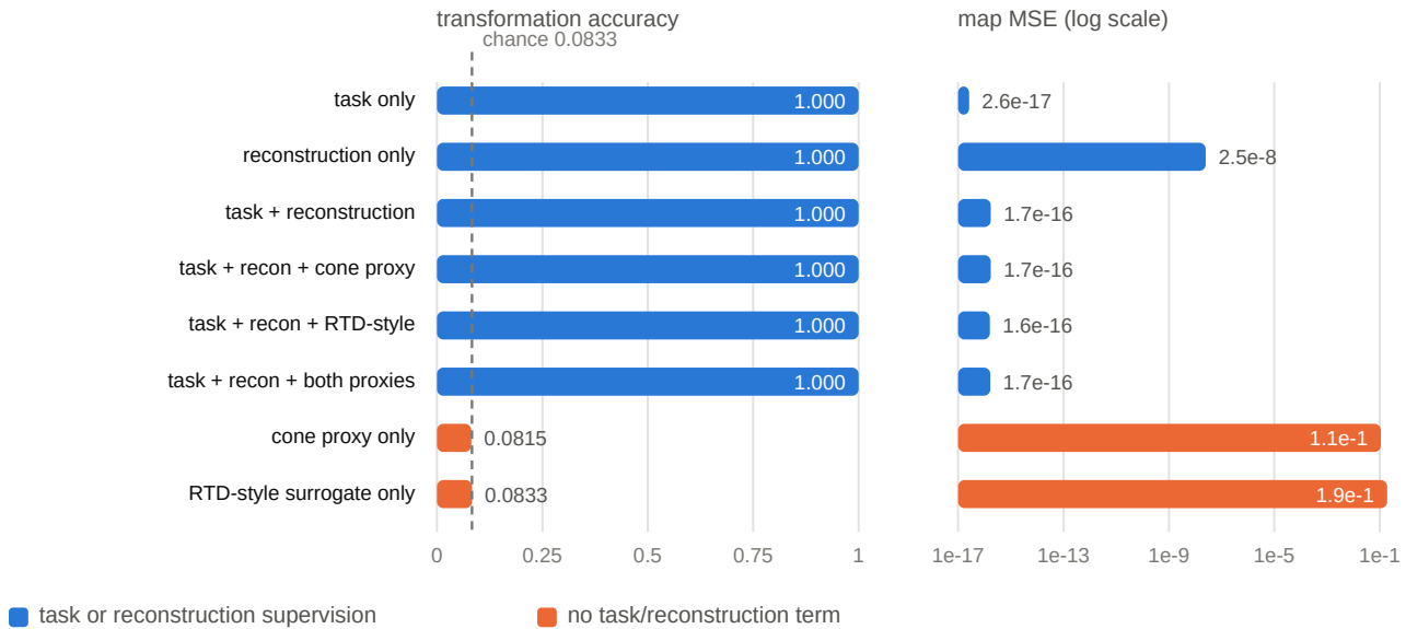
Figure 4. Recovery by objective in the selection setting. Mean over five seeds. All six objectives carrying task or reconstruction supervision have perfect decoded accuracy, with mean map MSE from 2.618\text{e-}17 to 2.504\text{e-}8 . The cone-only and RTD-only controls sit at chance with mean map MSE 0.109 and 0.191, about 7–16 orders of magnitude above the supervised range depending on the comparison. The RTD-only loss consumes target batch geometry and is not an unsupervised control. Generated from results/summaries/identifiable-campaign-summary.json .
