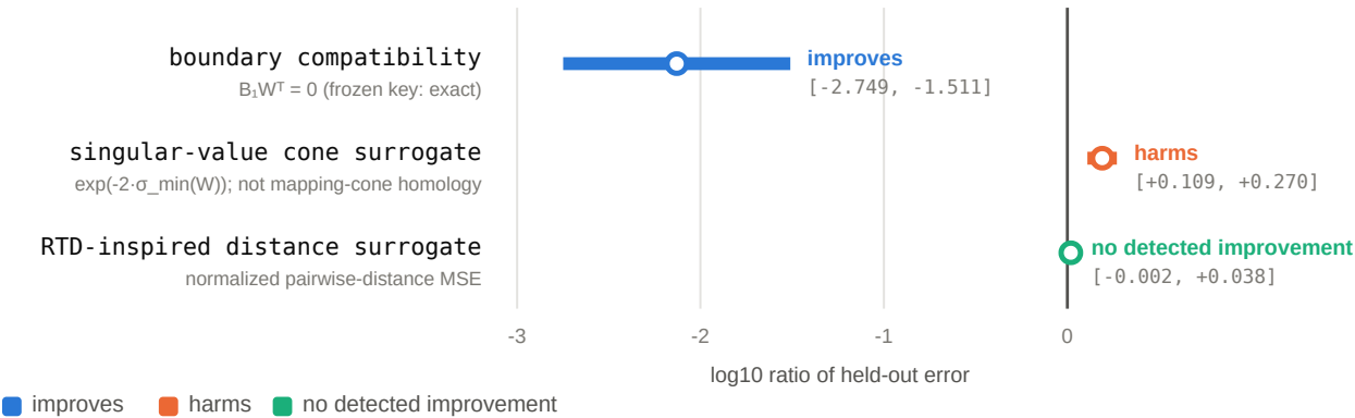
Figure 2. Three structural objectives under one protocol. Paired log10 (held-out error with term / without), one value per eligible generator seed, 29 joint topology/data/noise realizations. The thick bar is the Bonferroni-adjusted 98.33% interval governing the primary decision; the thin bar is the unadjusted 95% interval. Boundary compatibility improves held-out map recovery; the singular-value surrogate harms it; the RTD-inspired distance surrogate shows no detected improvement. The short labels in the graphic reproduce frozen campaign keys and do not identify exact with sequence exactness, cone with mapping-cone homology, or rtd with published RTD. Generated from results/campaigns/conversion-campaign-v1-corrected.json.
