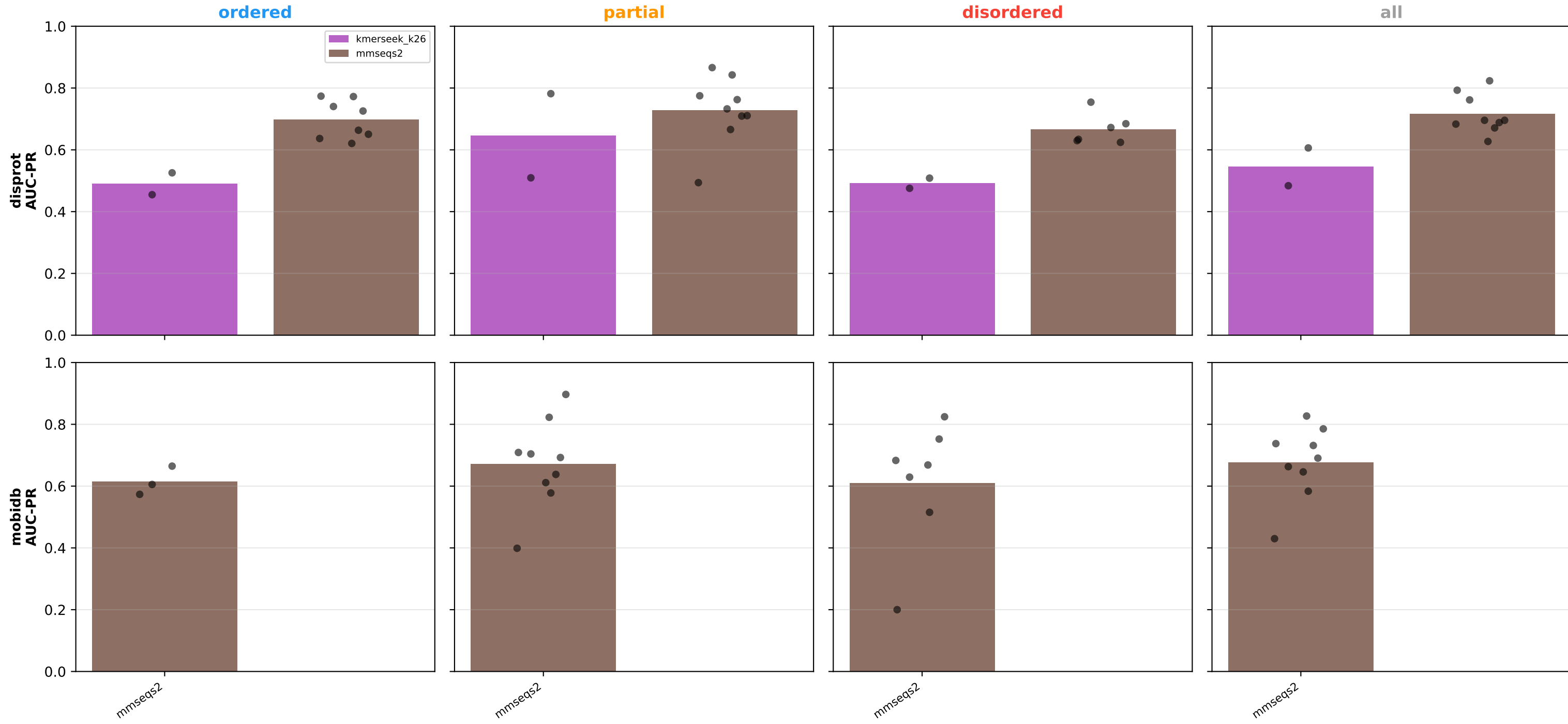
AUC-PR by tool, disorder category, and database (bars = mean across species; dots = individual species)
