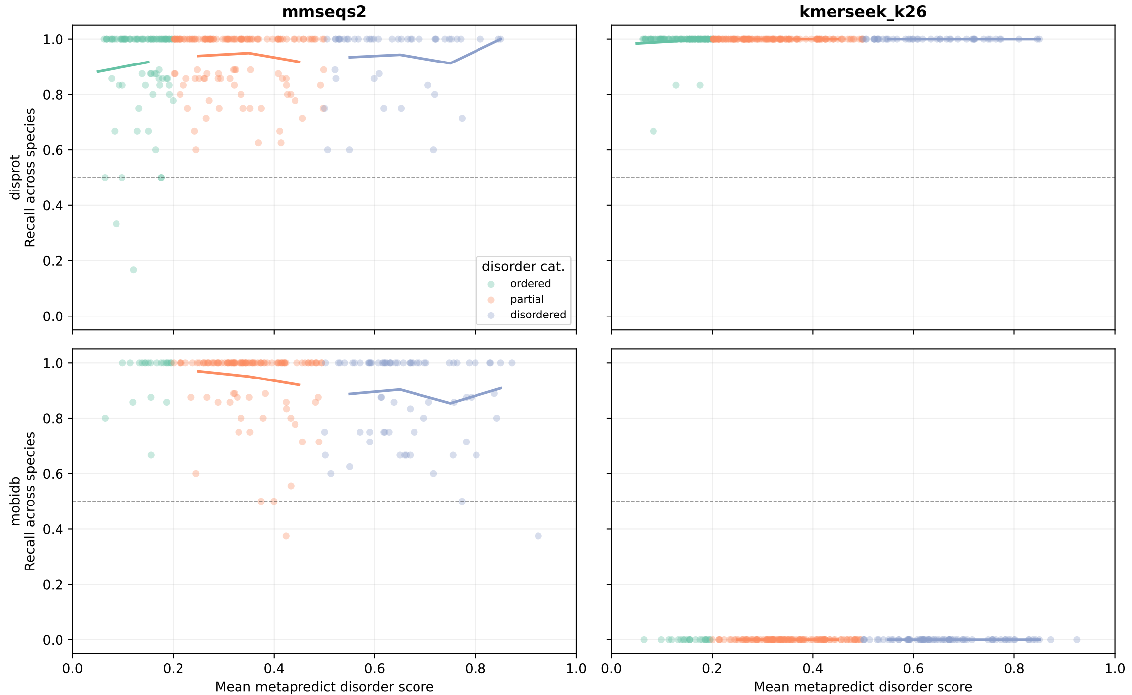
Per-protein recall vs disorder score (recall = fraction of positive species where tool found any hit; lines = binned means)
