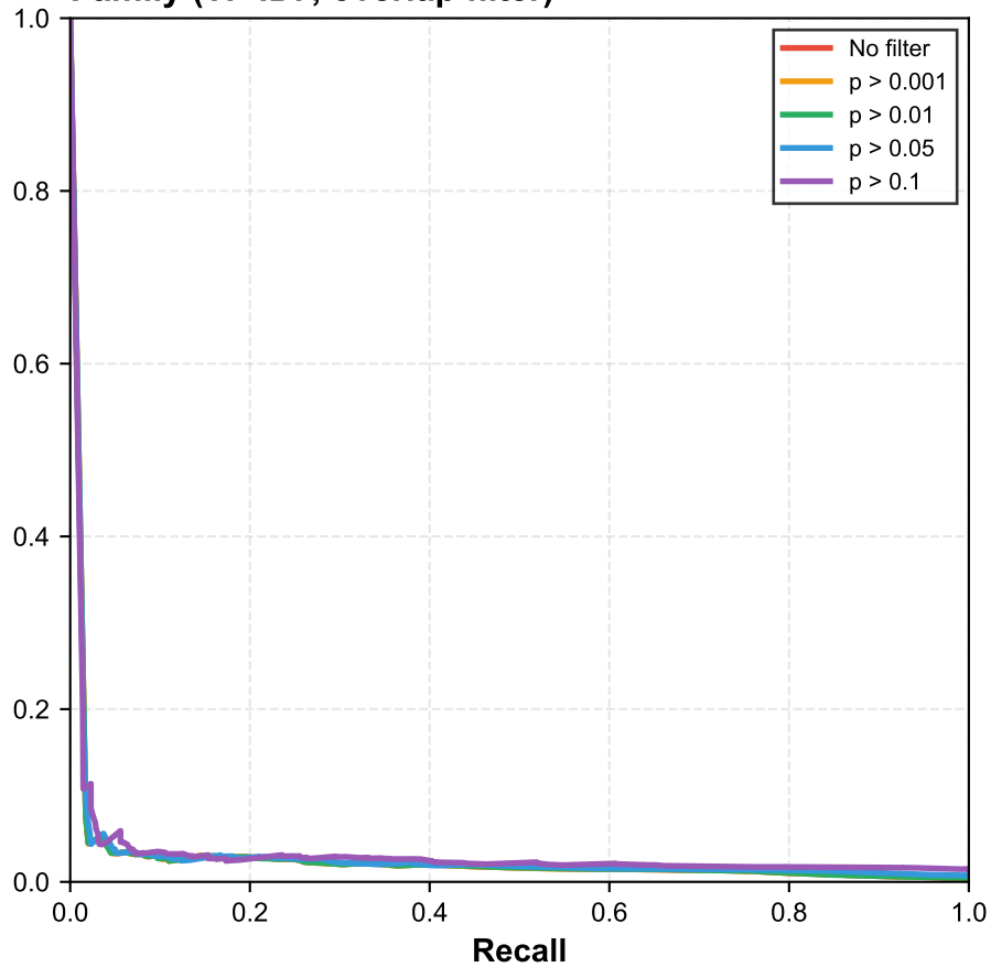
Family (TF-IDF, overlap filter)
