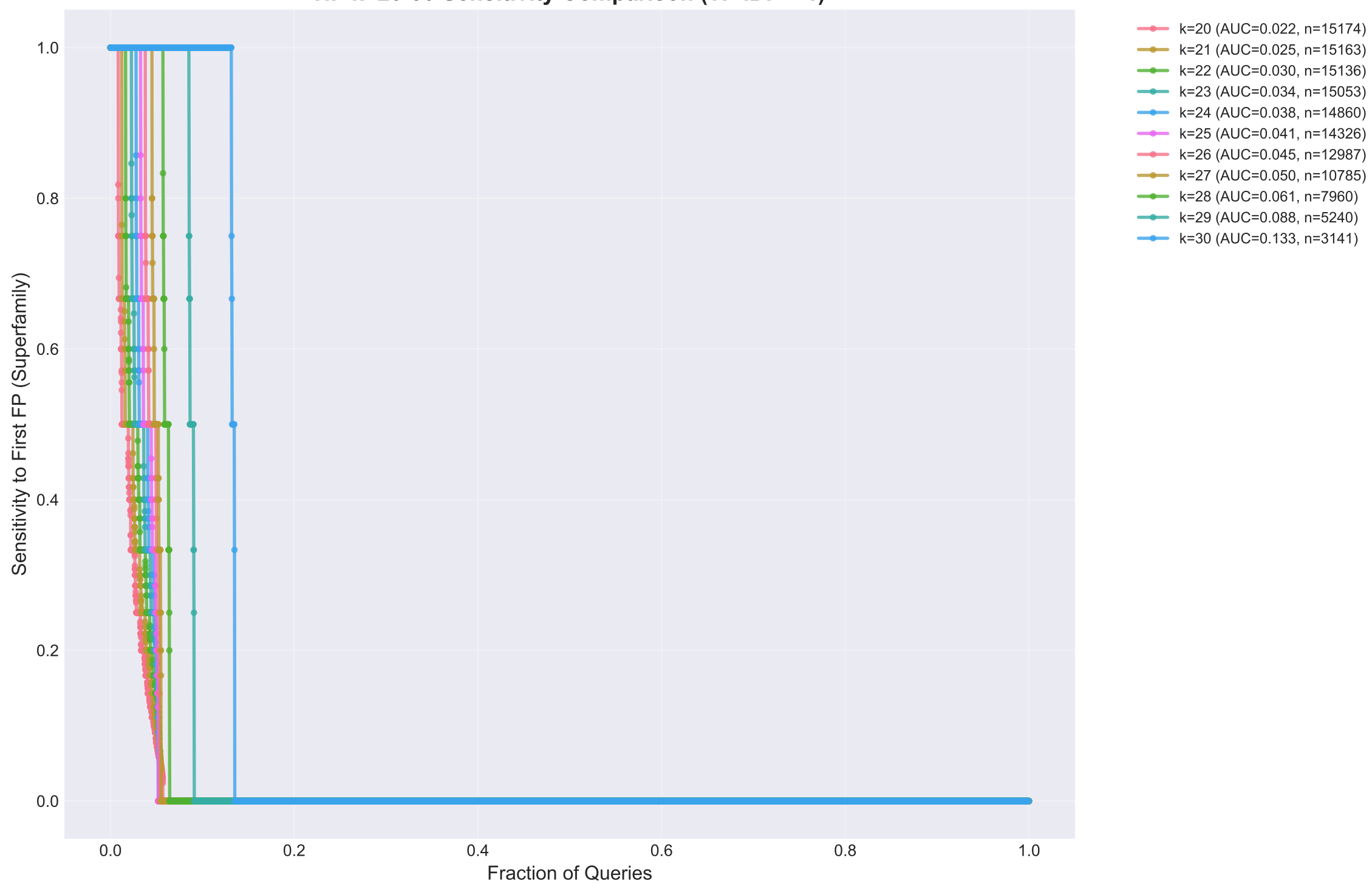
HP k=20-30 Sensitivity Comparison (TF-IDF > 1)
