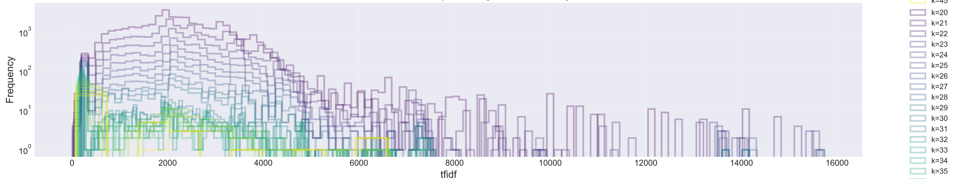
tfidf Distribution - Superfamily Matches Only
