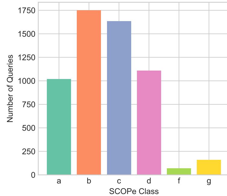
TEA (5737 total)
