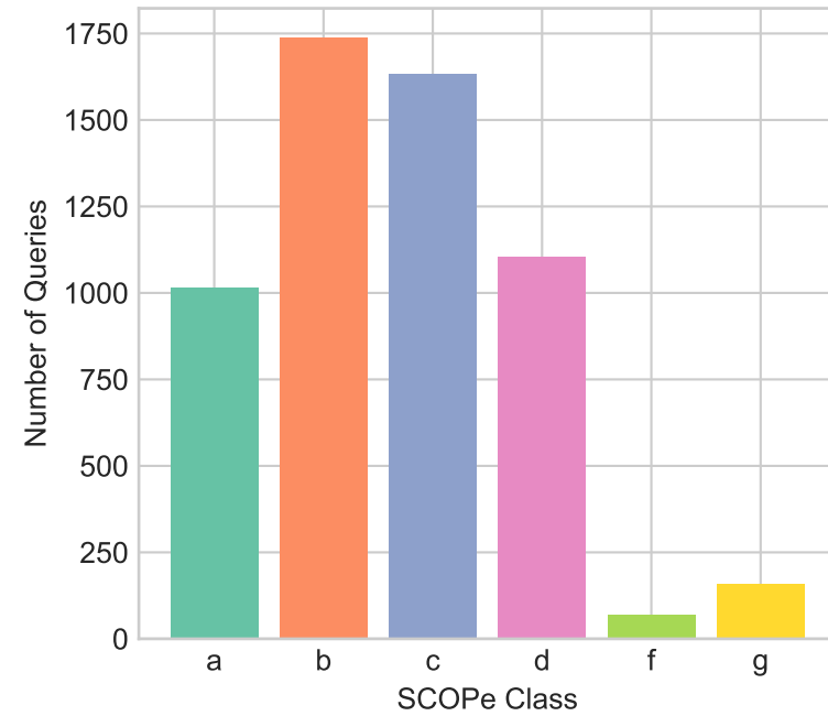
FoldSeek (5713 total)
