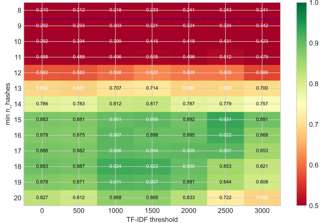
AUC (target = 0.580)
