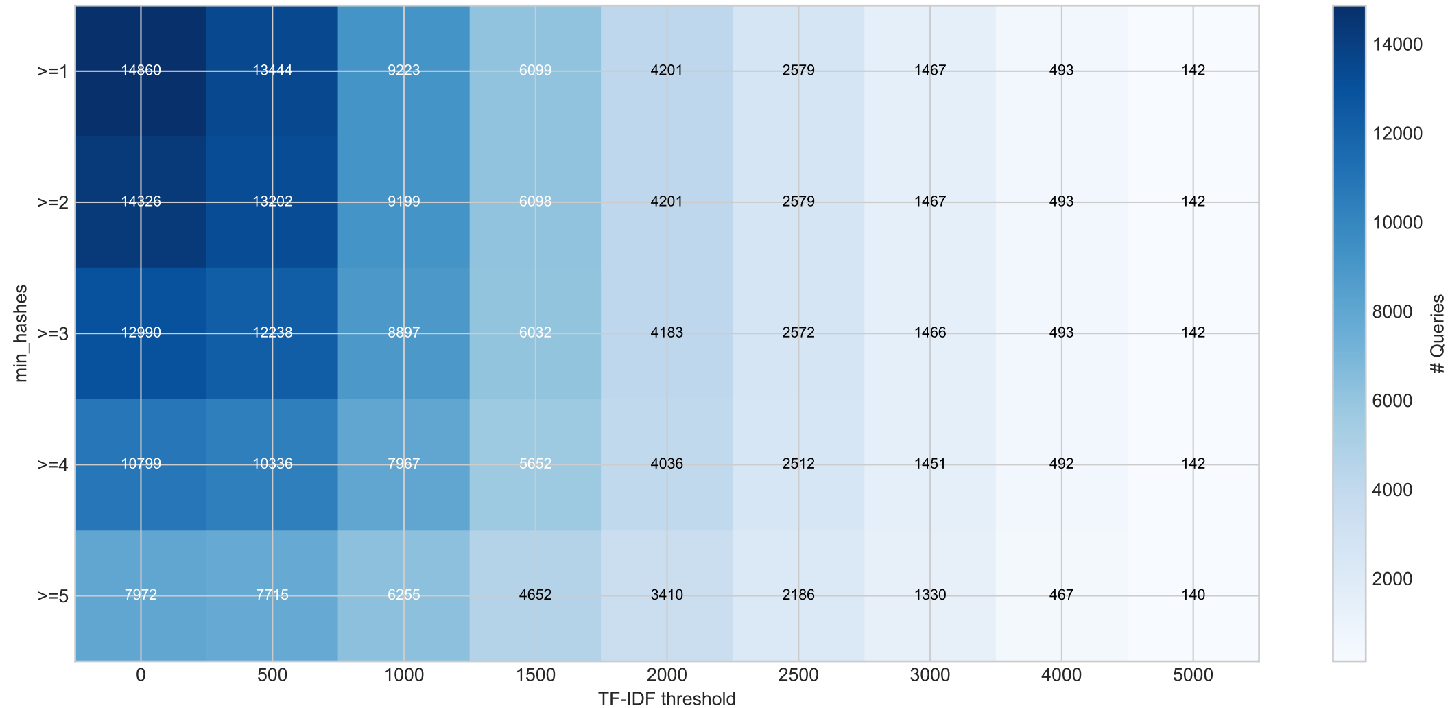
Grid Search: Query Counts (HP k=24)
