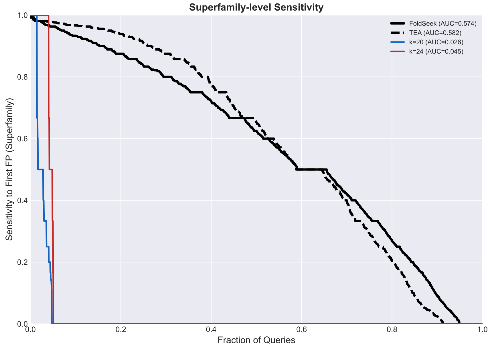
KmerSeek HP vs TEA vs FoldSeek — SCOPe40 (same query set, BH p-value) Note: all p-value correction methods give identical sensitivity curves (monotonic rank)
