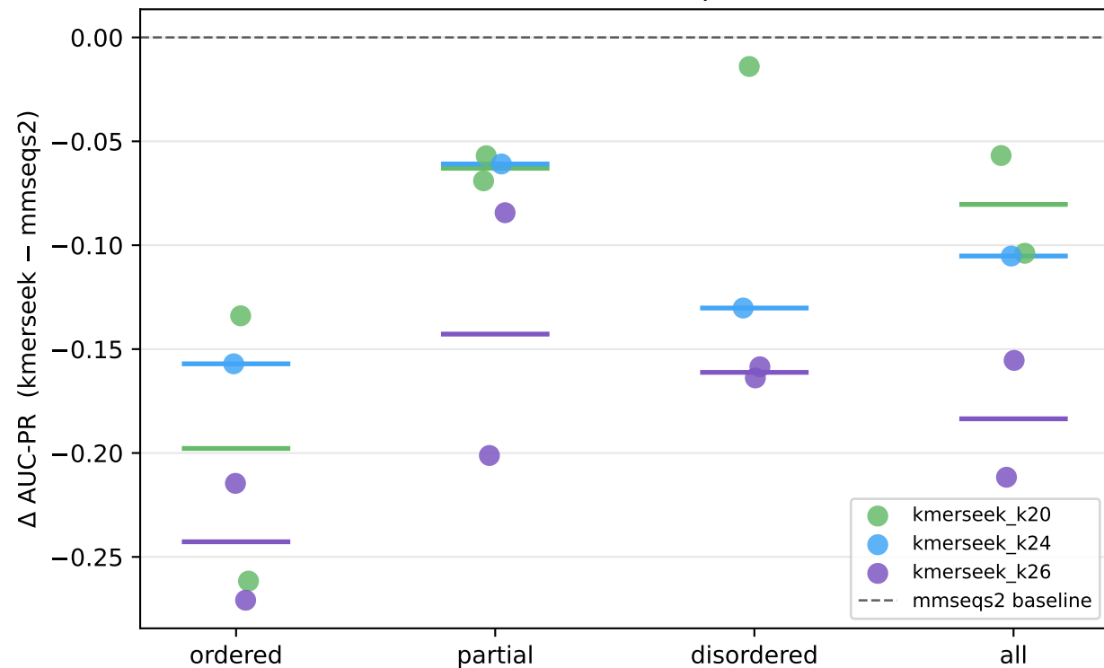
Kmerseek advantage by disorder category (each dot = one species)
