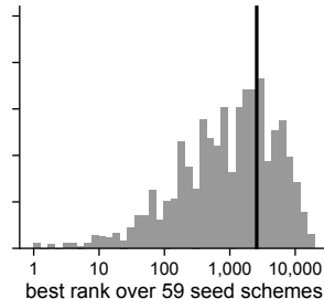
c P66: CD47, hp_thomas_dill2 rank 2,578; random as good: 69%
