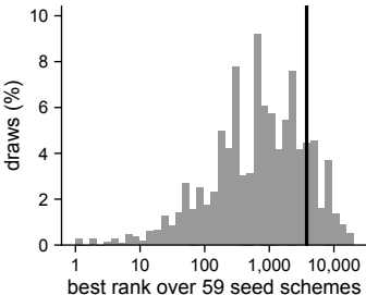
a CED-9: BCL2, hp_thomas_dill2 rank 3,788; random as good: 85%
