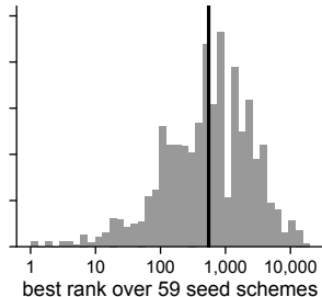
b CED-9: BCL2, hp_lehninger2 rank 551; random as good: 49%
