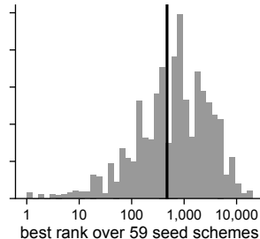
d P66: CD47, hp_lehninger2 rank 472; random as good: 41%
