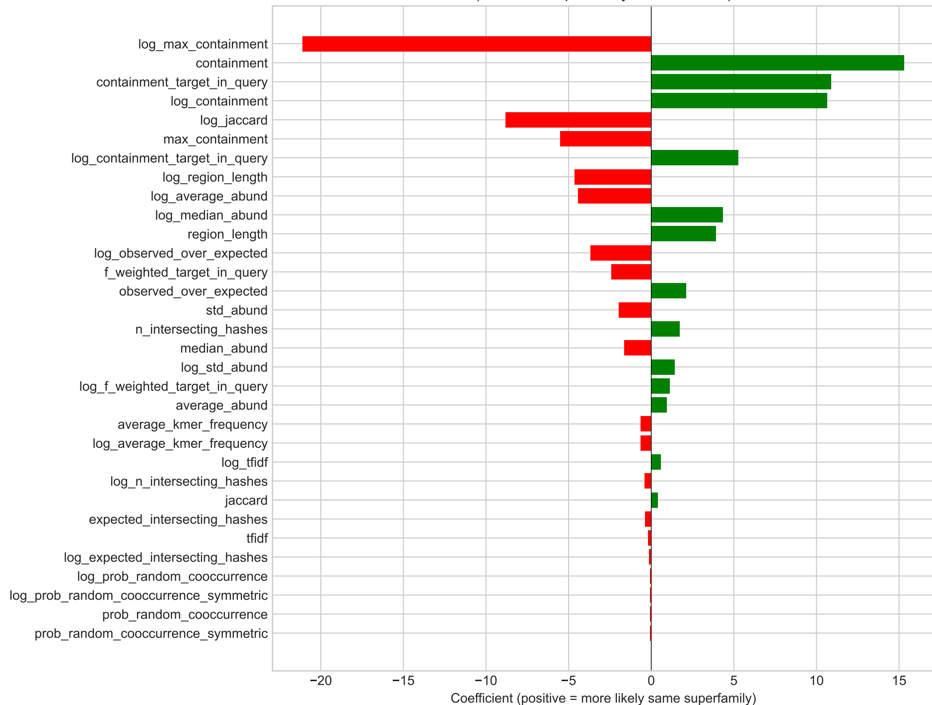
Logistic Regression Feature Importance (HP k=24 Superfamily Classification)
