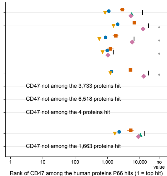
b query P66, target GENCODE v49 human proteome
