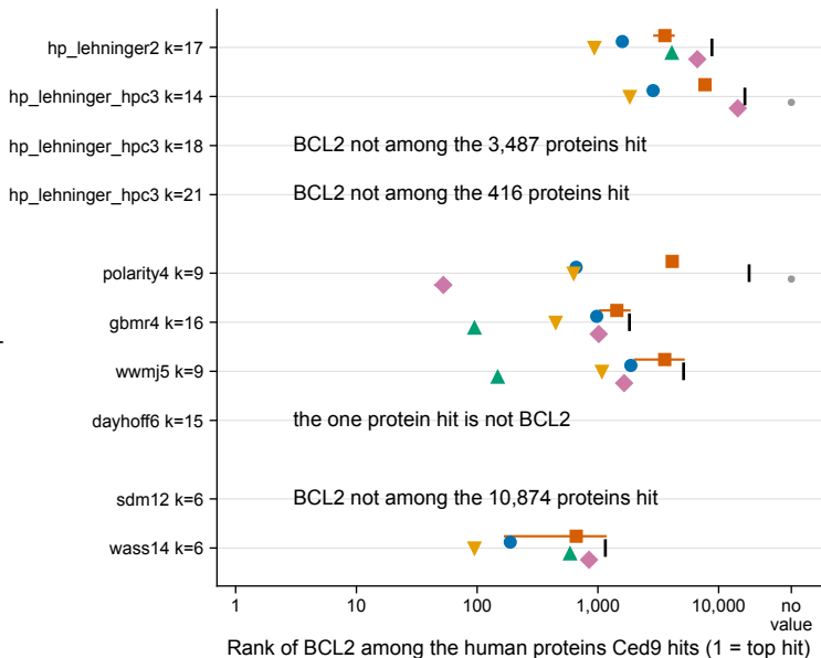
a query Ced9, target GENCODE v49 human proteome
