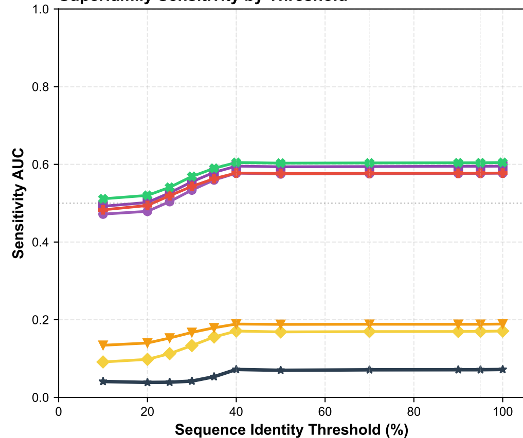
Superfamily Sensitivity by Threshold
