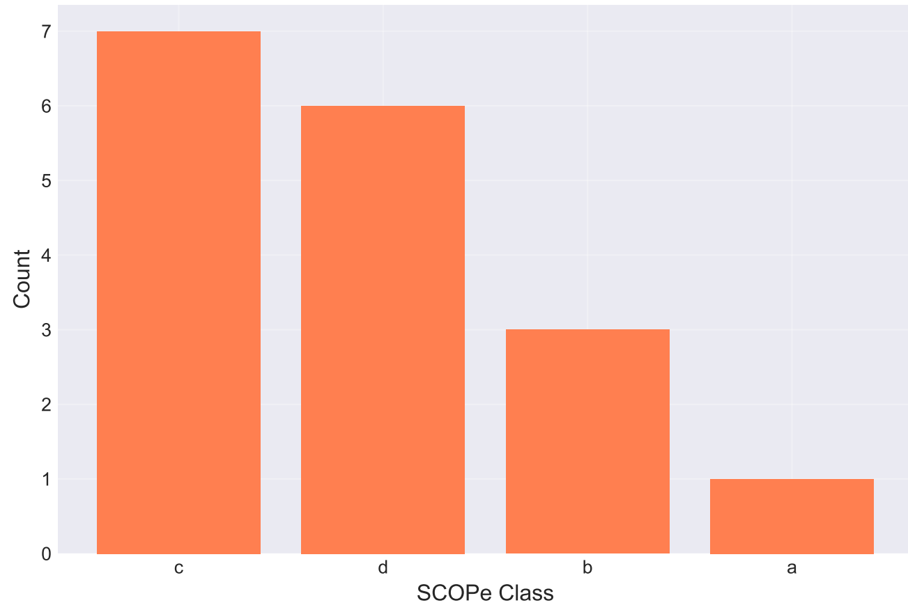
Unique to HP k=41 (n=17)
