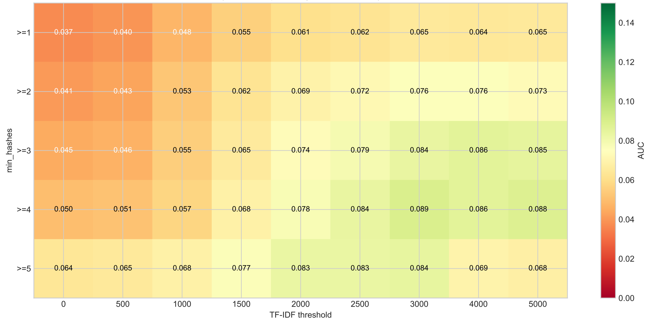
Grid Search: min_hashes x TF-IDF threshold (AUC at Superfamily level, HP k=24)
