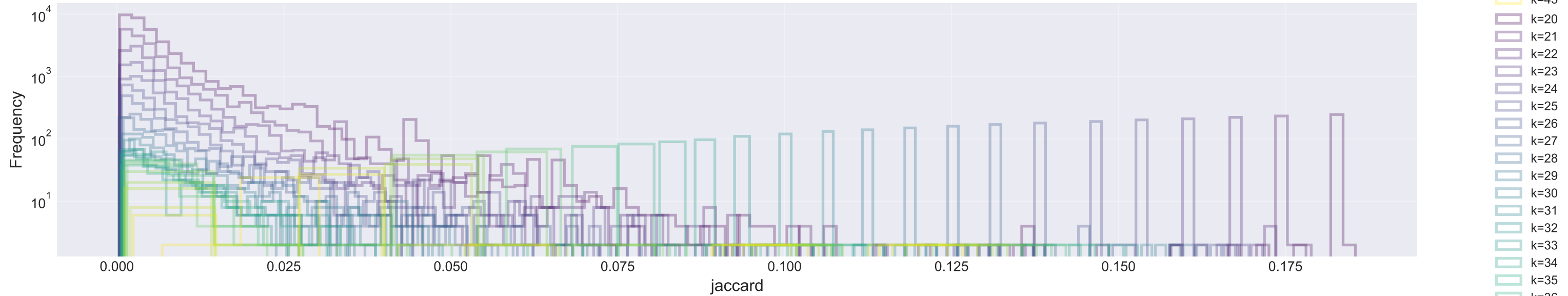
jaccard Distribution - Superfamily Matches Only
