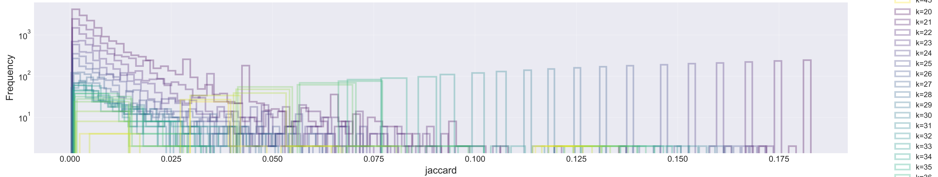
jaccard Distribution - Family Matches Only
