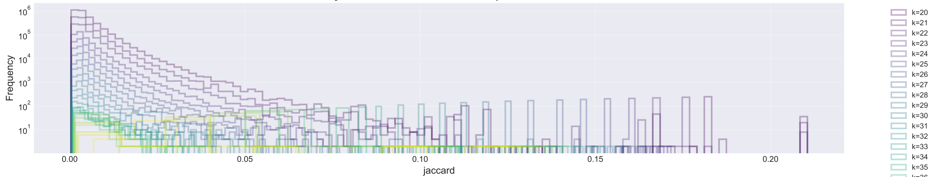
jaccard Distribution - All Comparisons
