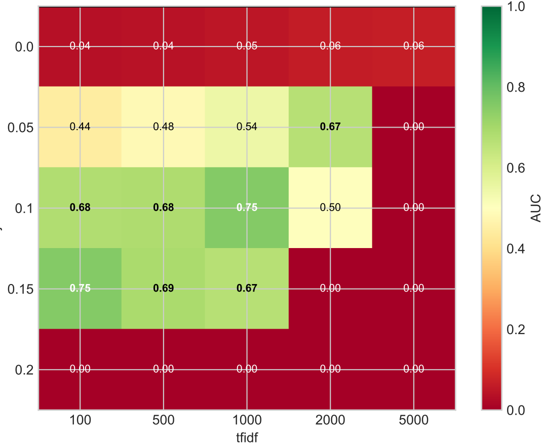
TF-IDF + Jaccard
