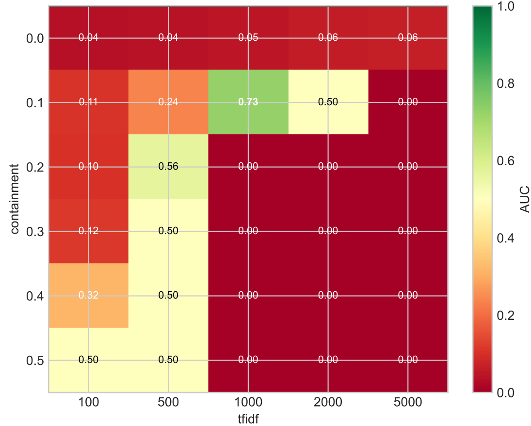
TF-IDF + Containment
